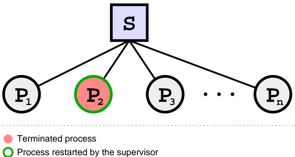
Figure 5.1: One_For_One Supervision
